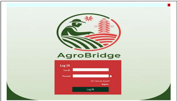
Fig1: Login Feature
