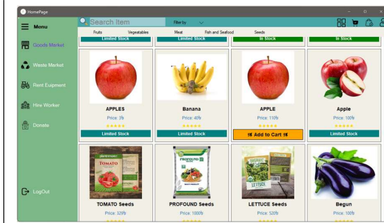
Fig3: Food Market
