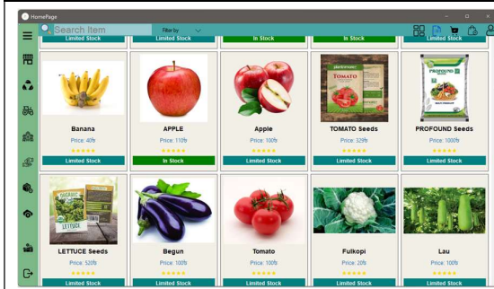
Fig3: Food Market
