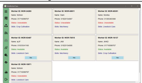
Fig6: Hire Worker
