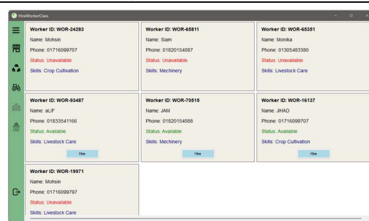
Fig6: Hire Worker
