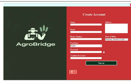
Fig2: Reg Feature
