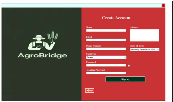
Fig2: Reg Feature
