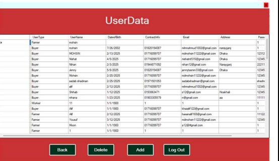
Fig4: User Info
