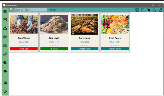
Fig4: Waste Market
