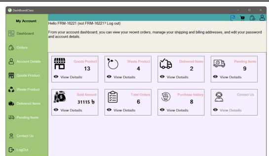
Fig14: Farmer Dashboard
