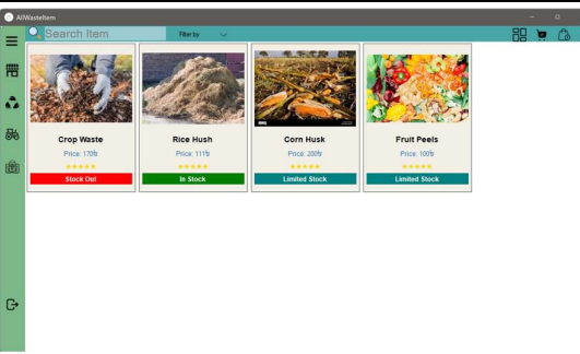
Fig4: Waste Market
