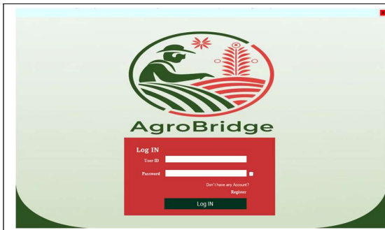
Fig1: Login Feature
