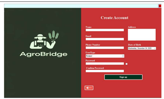
Fig2: Reg Feature
