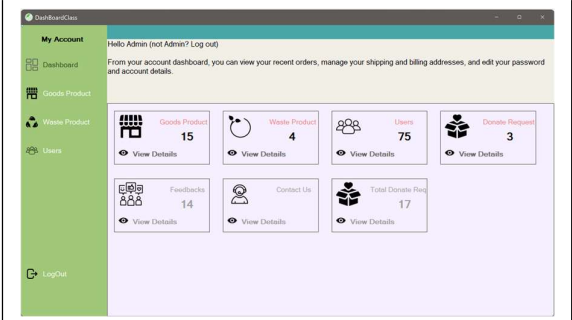
Fig3: Admin Dashboard
