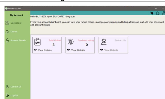
Fig8: Buyers Dashboard
