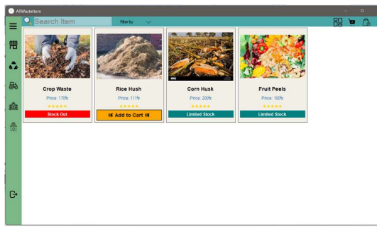
Fig4: Waste Market
